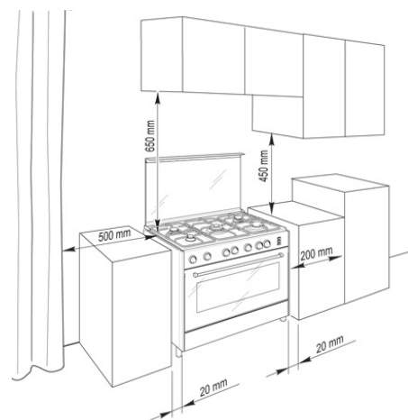
Technical Diagram
